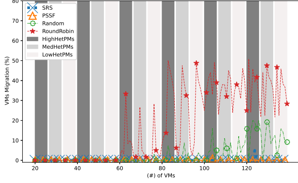
(a) Mig_{vms} for VMs Arrival Time: M(t) < T(t) < N(t)
