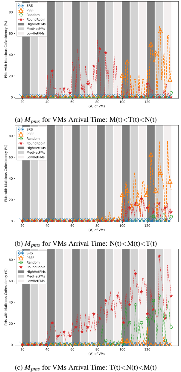
Figure 3: Comparison of percentage of the malicious co-residency under three arrivals times for M(t), T(t) and N(t) .
