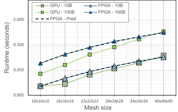
Figure 7: RTM forward-pass, FP32, p = 2, v = 3, 200 iterations
